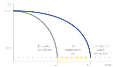
Figure 3. Benefit of continuous online drying system
